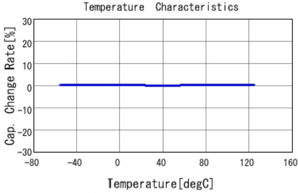
GRM1555C1H4R7CA01 C-Temp. capchange, DCOV, AC1Vrms
