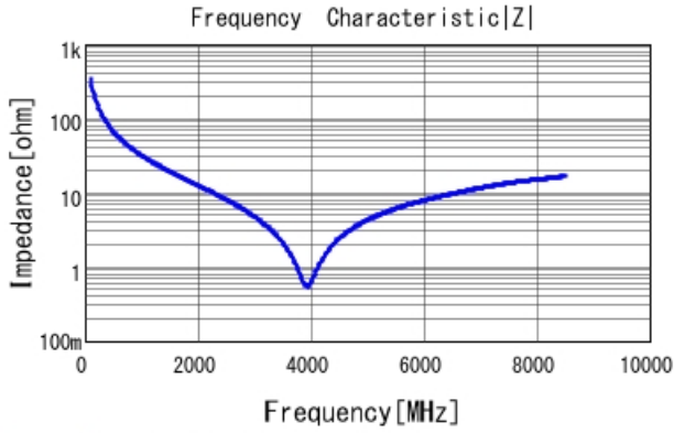
GRM1555C1H4R7CA01 |Z| DCOV, 25degC
