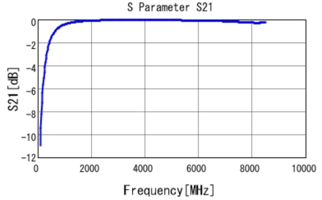
GRM1555C1H4R7CA01 S21 DCOV, 25degC
