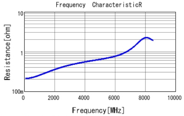
GRM1555C1H4R7CA01 R DCOV, 25degC
