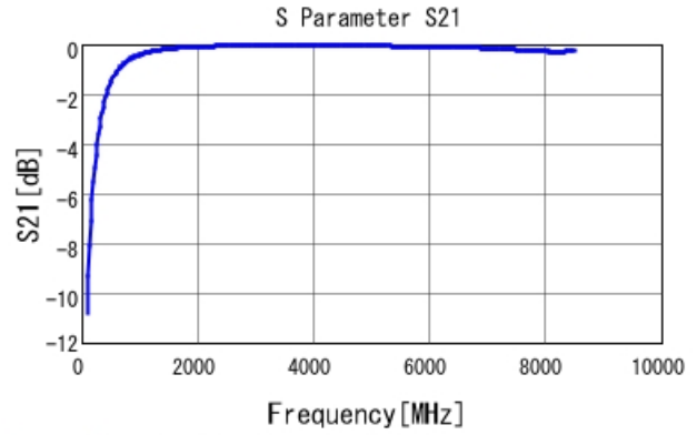
GRM1555C1H4R8WA01 S21 DCOV, 25degC
