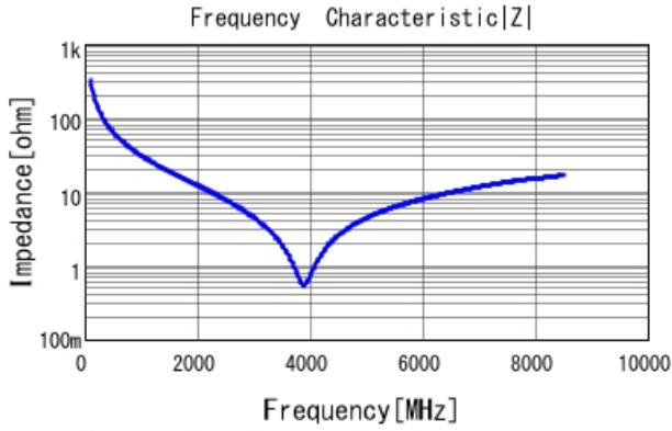
GRM1555C1H4R8WA01 |Z| DCOV, 25degC
