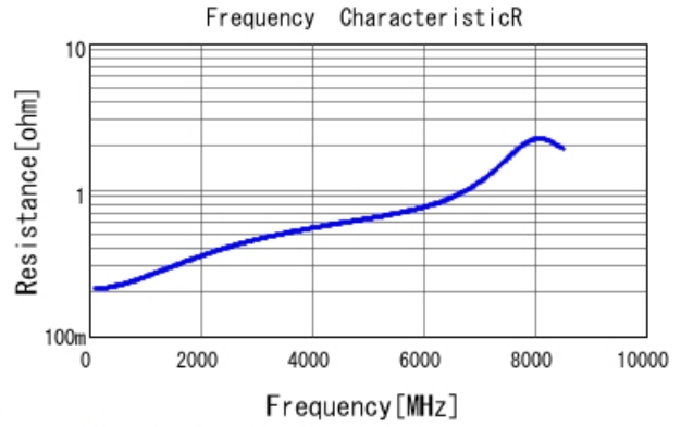
GRM1555C1H4R8WA01 R DCOV, 25degC
