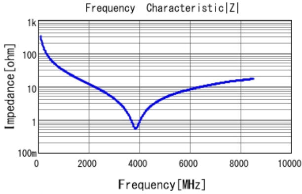
GRM1555C1H4R9BA01 |Z| DCOV, 25degC
