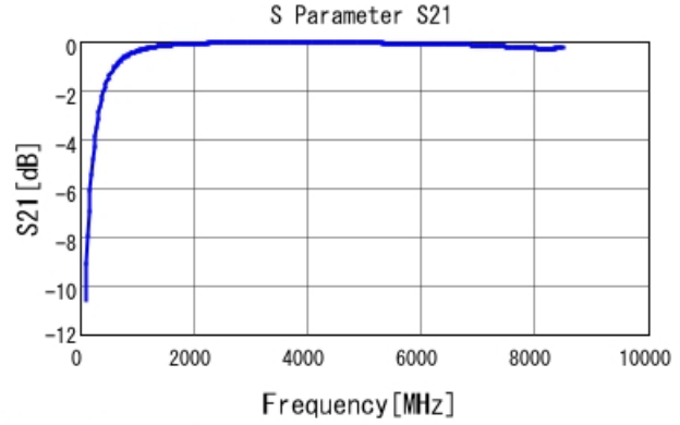
GRM1555C1H4R9BA01 S21 DC0V, 25degC
