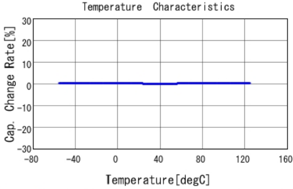
GRM1555C1H4R9BA01 C-Temp. capchange, DC0V, AC1Vrms
