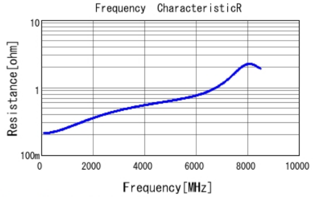
GRM1555C1H4R9BA01 R DCOV, 25degC
