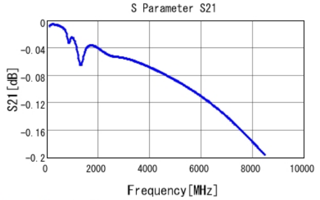
GRM1555C1H511GA01 S21 DCOV, 25degC
