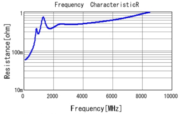
GRM1555C1H511GA01 R DCOV, 25degC
