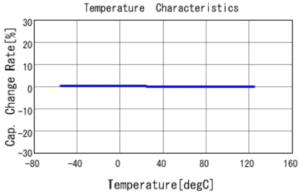
GRM1555C1H511GA01 C-Temp. capchange, DCOV, AC1Vrms
