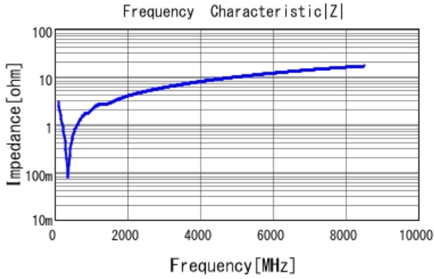
GRM1555C1H511GA01 |Z| DCOV, 25degC
