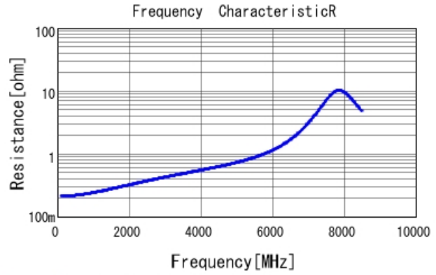
GRM1555C1H5R0CA01 R DCOV, 25degC
