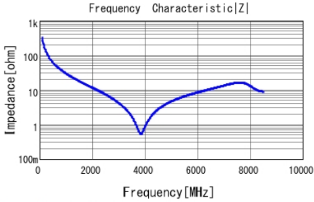
GRM1555C1H5R0CA01 |Z| DCOV, 25degC
