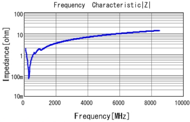
GRM1555C1H751GA01 |Z| DCOV, 25degC
