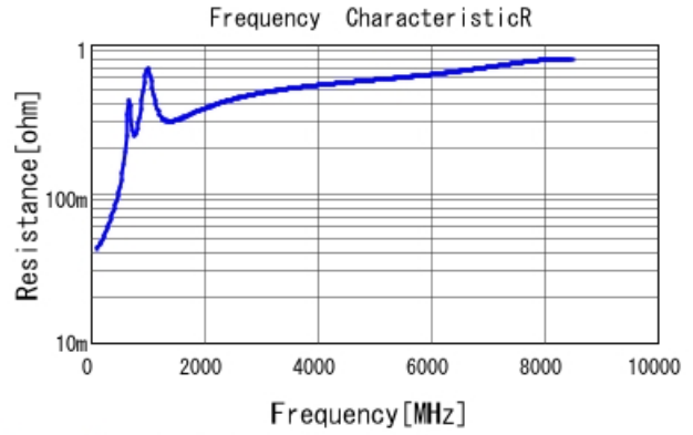
GRM1555C1H751GA01 R DCOV, 25degC
