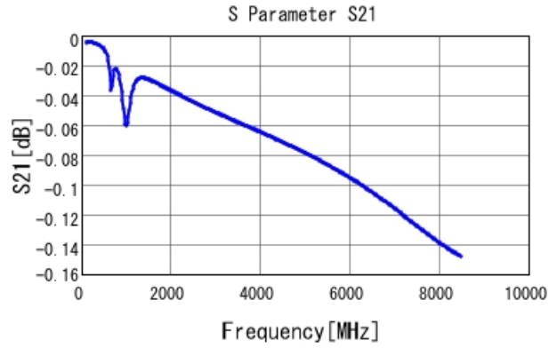
GRM1555C1H751GA01 S21 DCOV, 25degC
