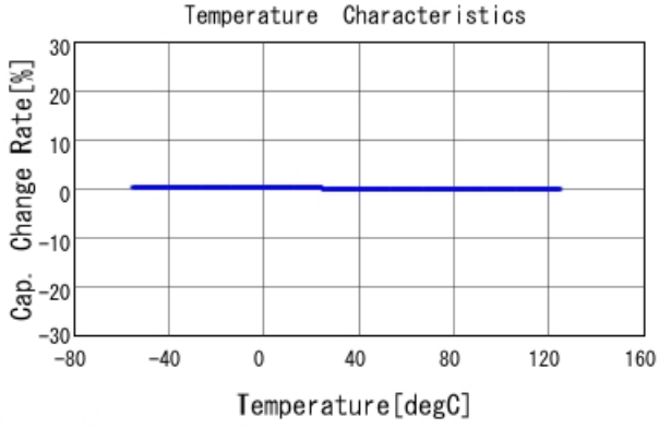
GRM1555C1H822JE01 C-Temp. capchange, DCOV, AC1Vrms
