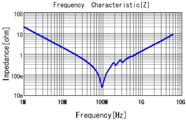
GRM1555C1H822JE01 |Z| DCOV, 25degC
