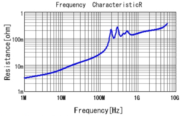
GRM1555C1H822JE01 R DCOV, 25degC
