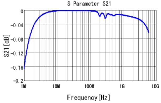
GRM1555C1H822JE01 S21 DCOV, 25degC
