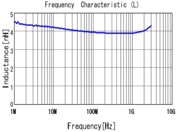
■ LQW15AN4N0G80 L
