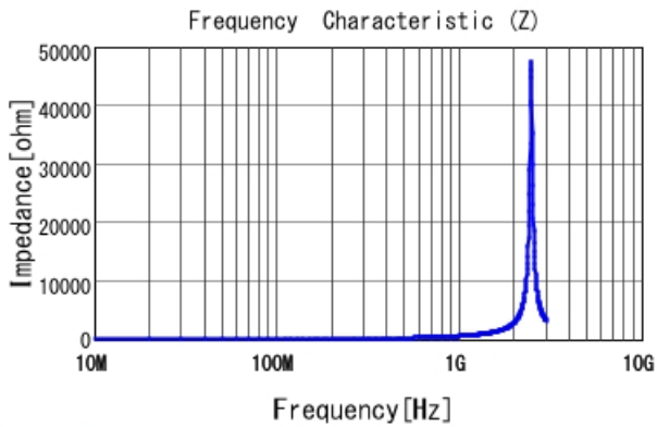
LQW18AN82NJ00 |Z|
