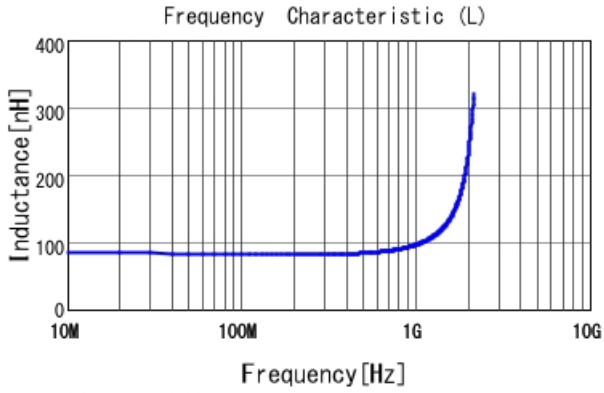
LQW18AN82NJ00 L
