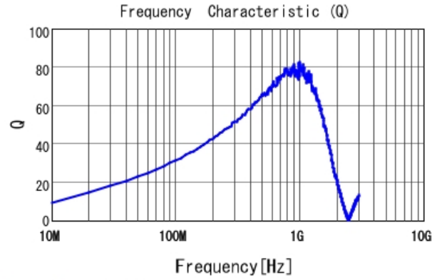
LQW18AN82NJ00 Q
