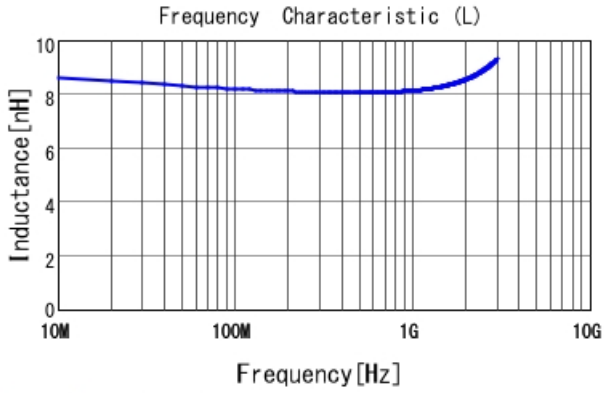
LQW18AN8N2D00 L
