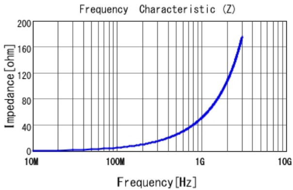
LQW18AN8N2D00 |Z|
