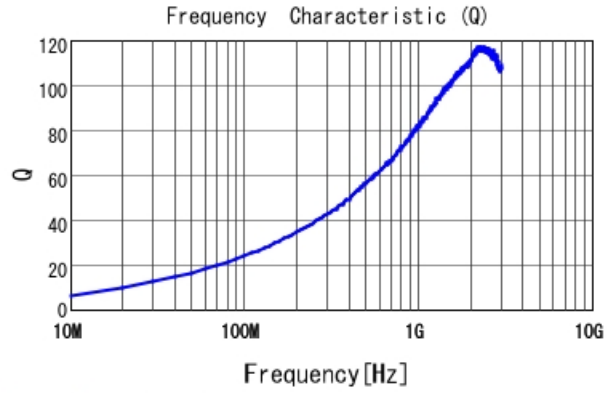
LQW18AN8N2D00 Q
