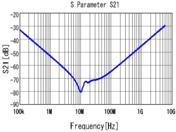
■ NFM21PC475B1A3 S21 DC0V, 25degC, Feedthrough
