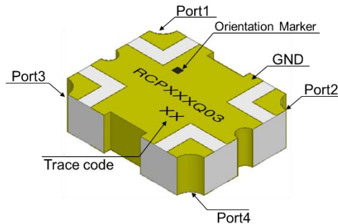
Figure 1. RCP2650Q03 (Top View)
