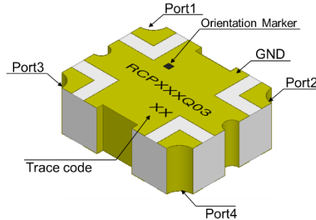
Figure 1. RCP890Q03 (Top View)
